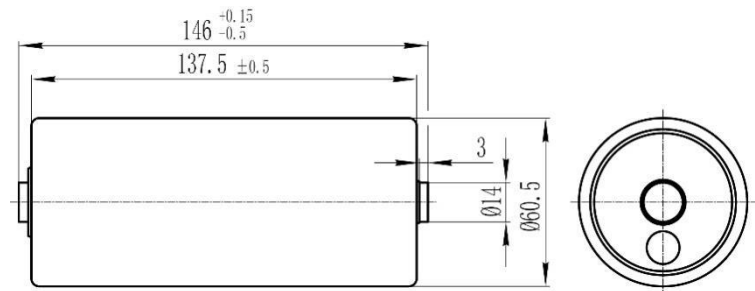
Dimension of UCK42V28000
