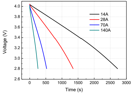
Discharge curves under 2.8 ~ 4.05V (left) and 2.8 ~ 3.8V (right) of UCK42V28000
