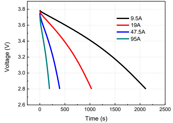
Discharge curves under 2.8 ~ 4.0V (left) and 2.8 ~ 3.8V (right) of UCK42V14000C
